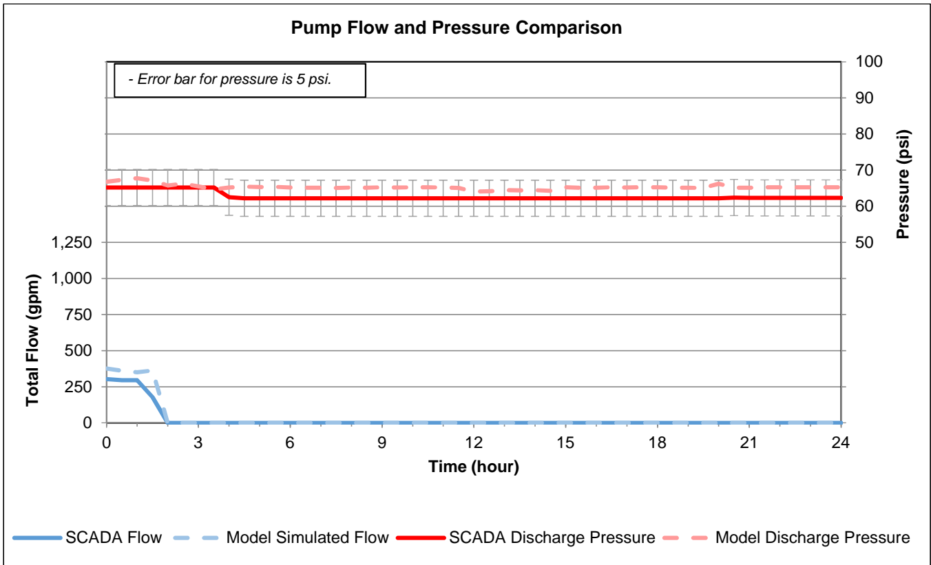
Figure 9. Tank 3 Comparison December 15, 2015
