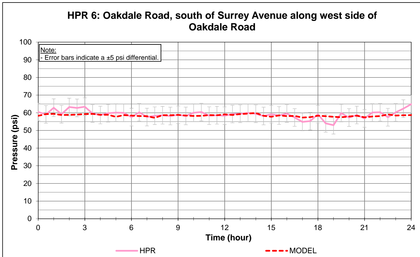
Figure 2. Round 2 HPR 6 and 9 December 15, 2015
