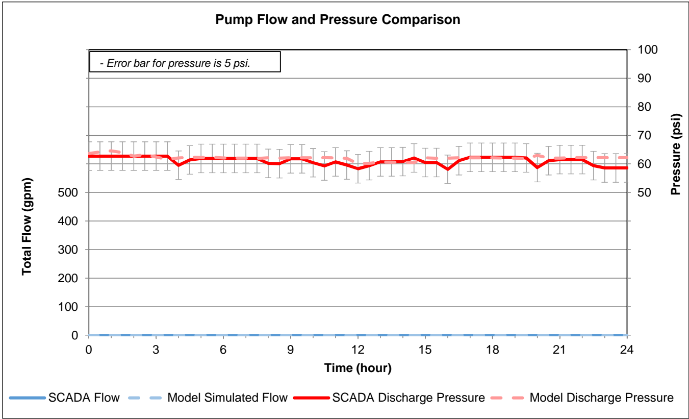
Figure 13. Tank 7 Comparison December 15, 2015
