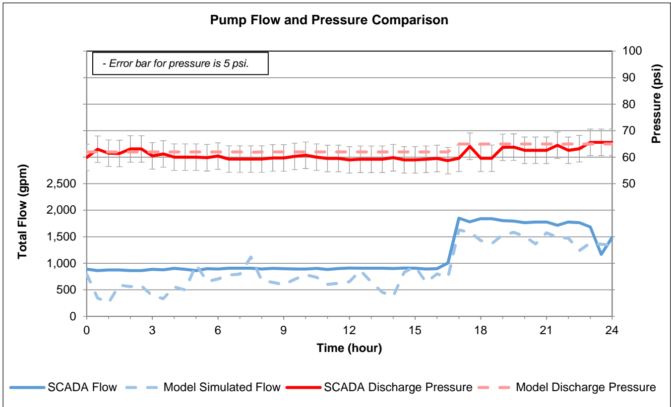
Figure 11. Tank 5 Comparison December 15, 2015
