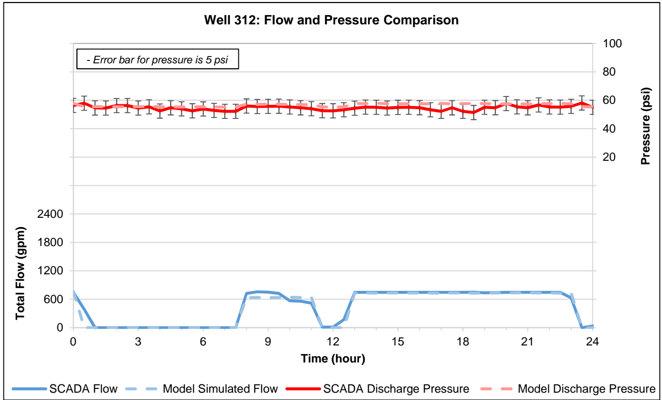
Figure 22. Well 312 December 15, 2015
