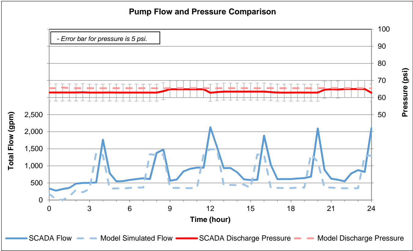
Figure 12. Tank 6 Comparison December 15, 2015
