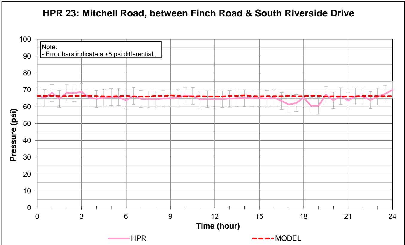
Figure 5. Round 2 HPR 23 and 24 December 15, 2015
