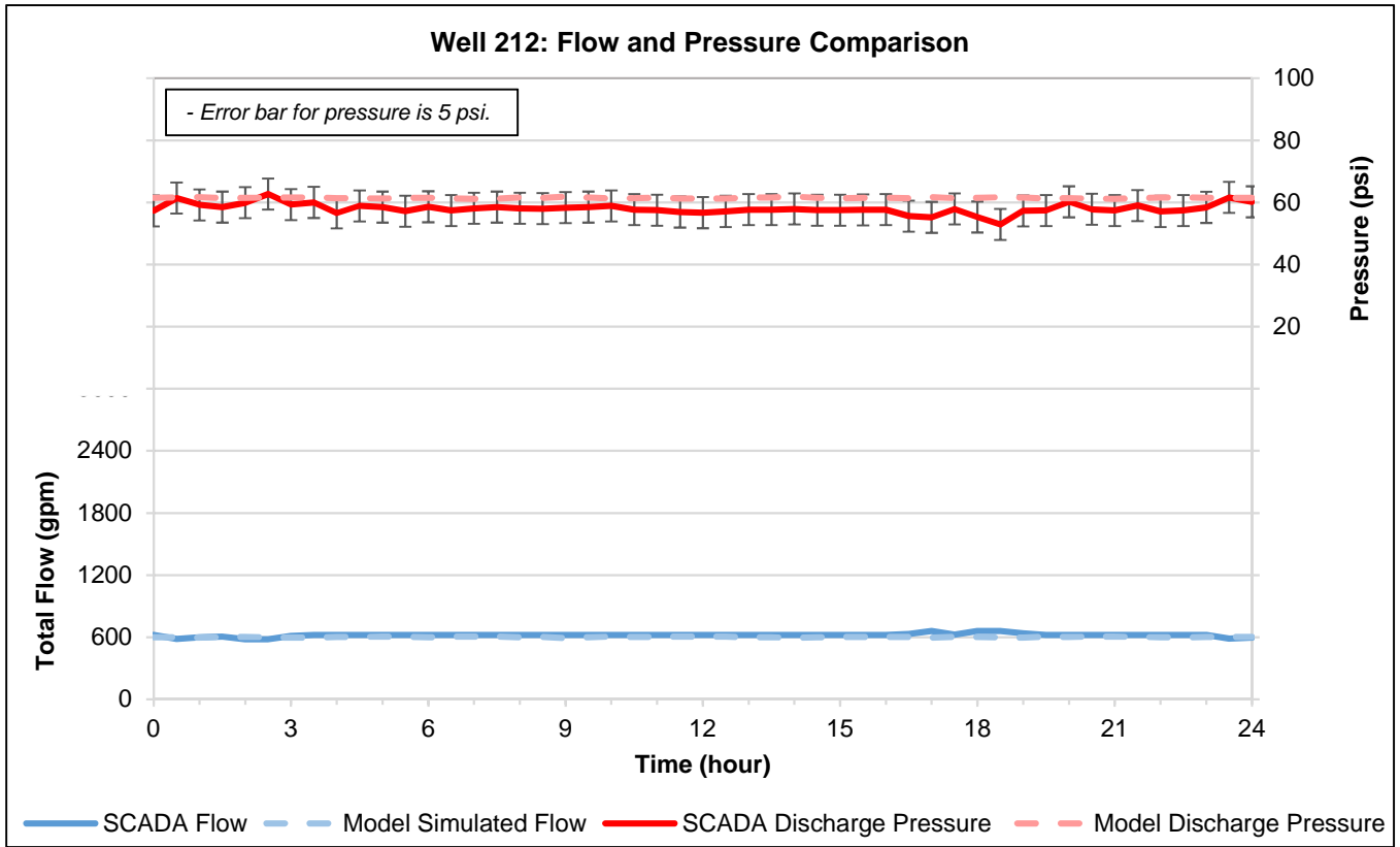
Figure 19. Well 212 and 225 December 15, 2015
