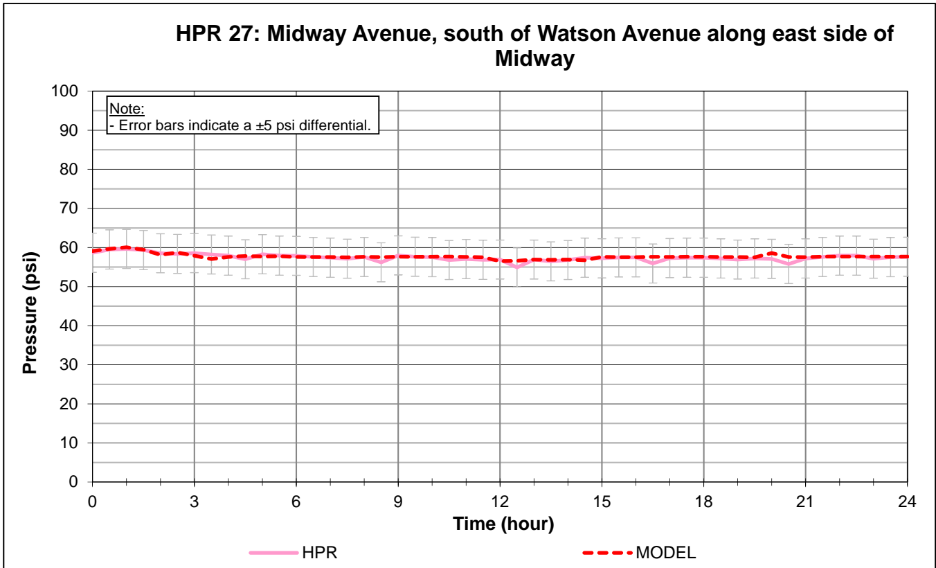
Figure 7. Round 2 HPR 27 and 28 December 15, 2015
