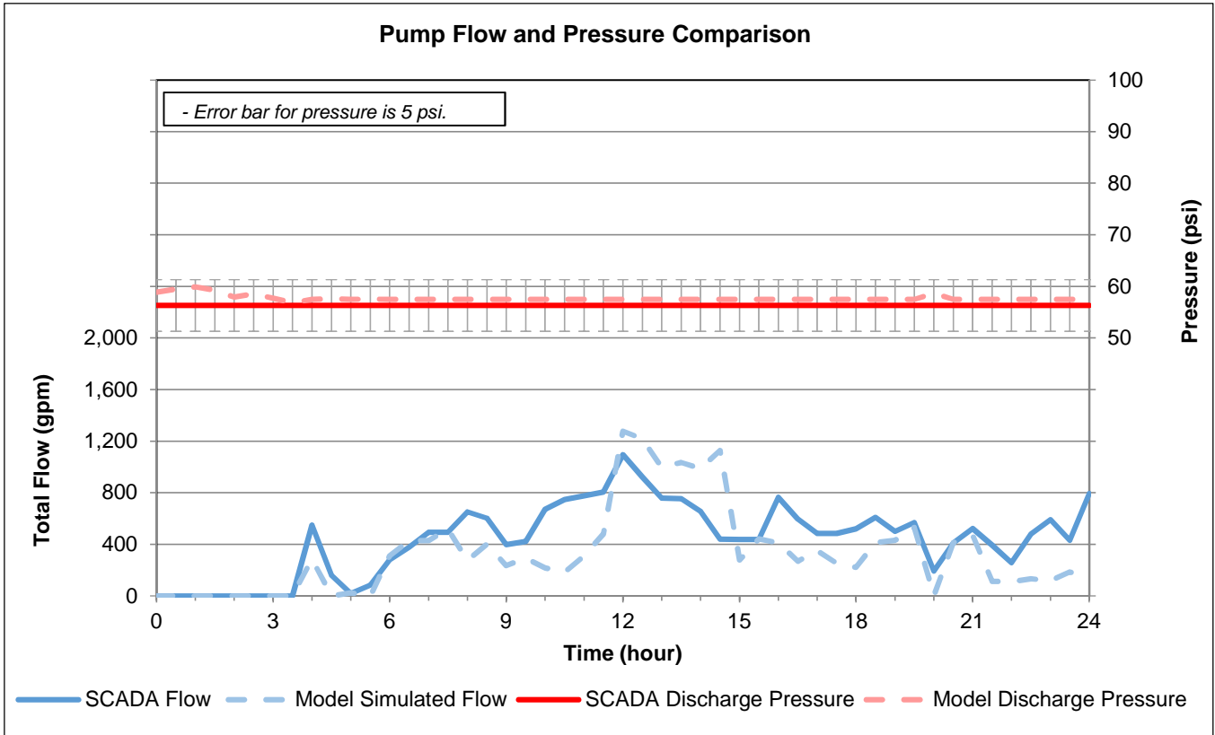
Figure 14. Tank 8 Comparison December 15, 2015
