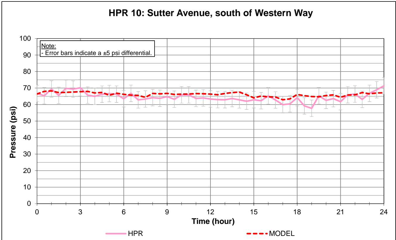
Figure 3. Round 2 HPR 10 and 11 December 15, 2015
