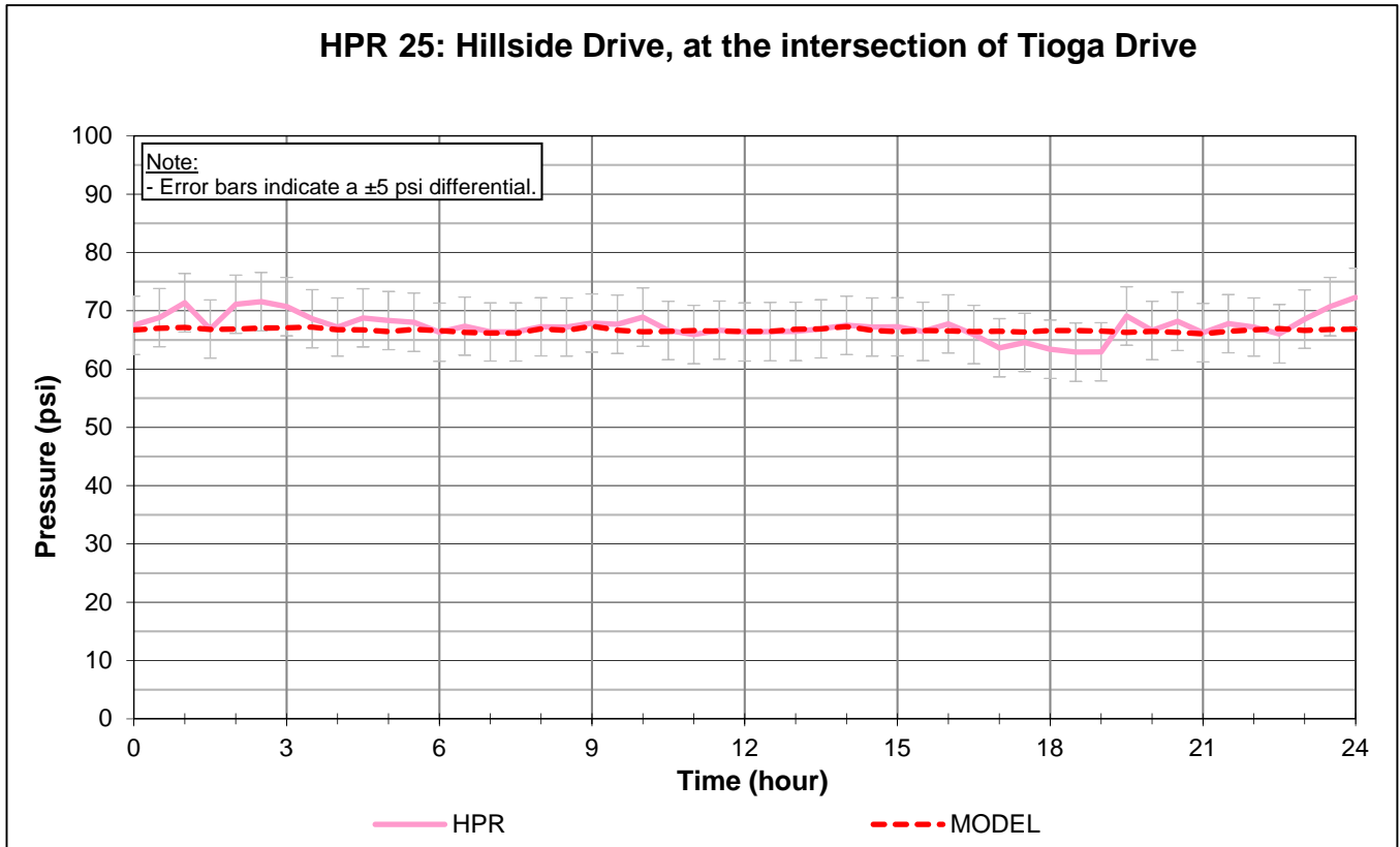
Figure 6. Round 2 HPR 25 and 26 December 15, 2015
