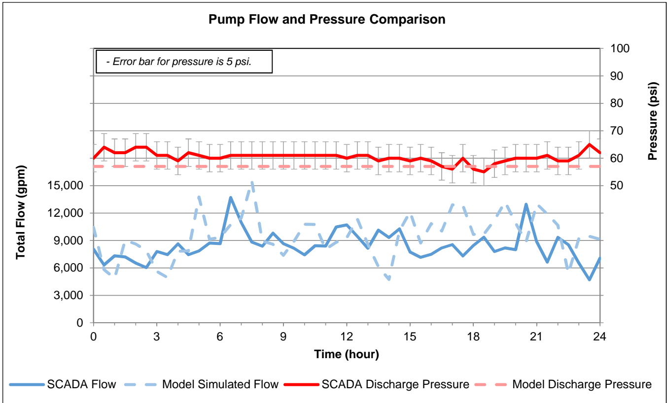
Figure 8. MID Tank Comparison December 15, 2015
