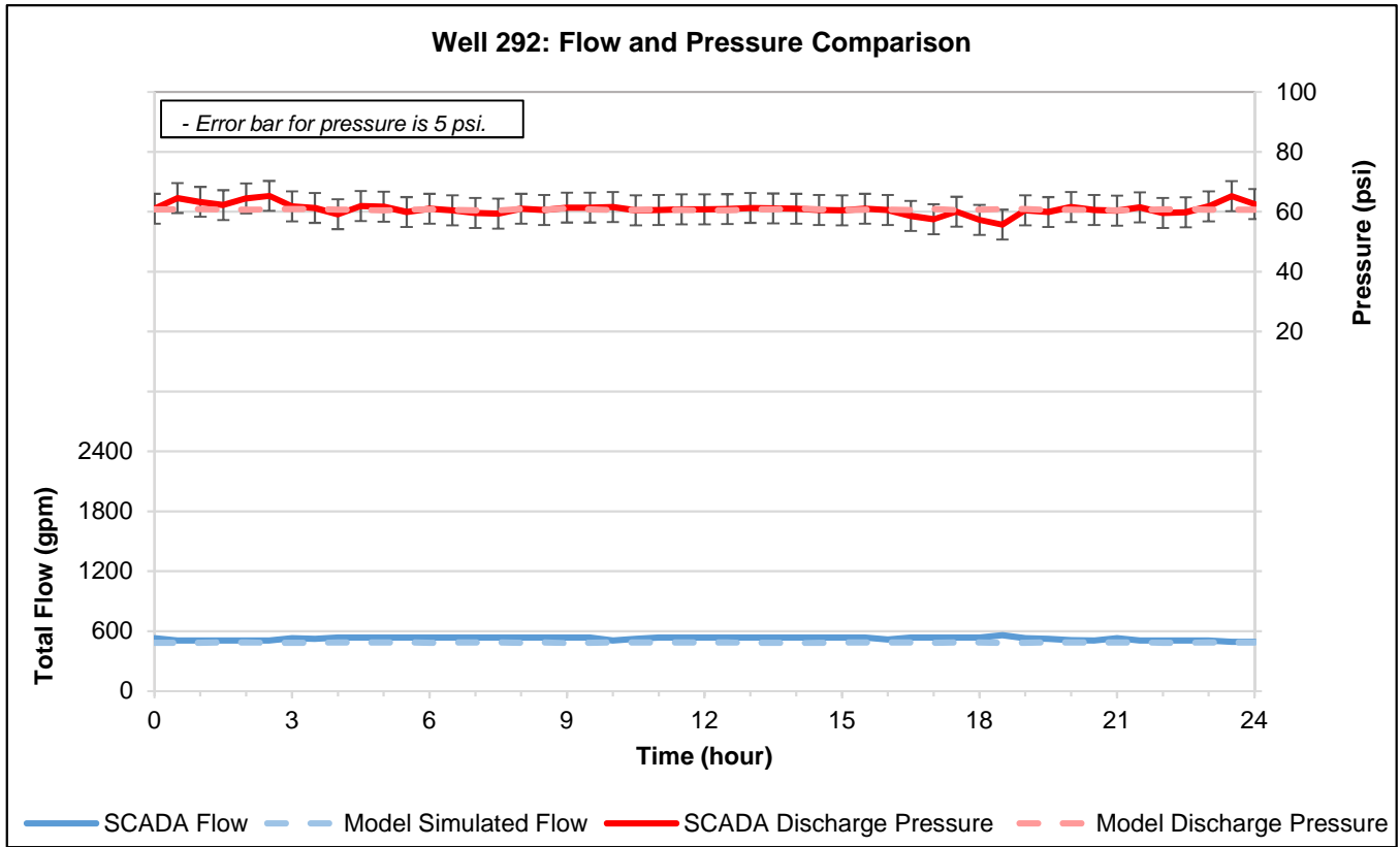
Figure 21. Well 292 and 297 December 15, 2015
