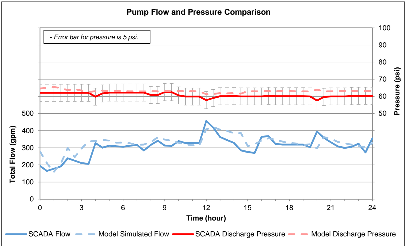
Figure 15. Tank 10 Comparison December 15, 2015
