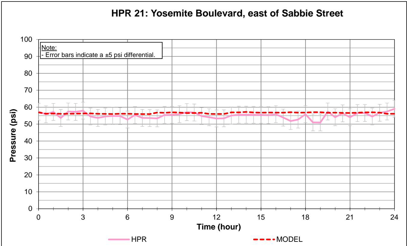
Figure 4. Round 2 HPR 21 and 22 December 15, 2015
