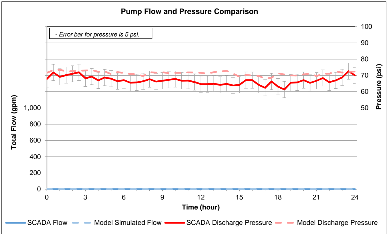
Figure 16. Tank 12 Comparison December 15, 2015
