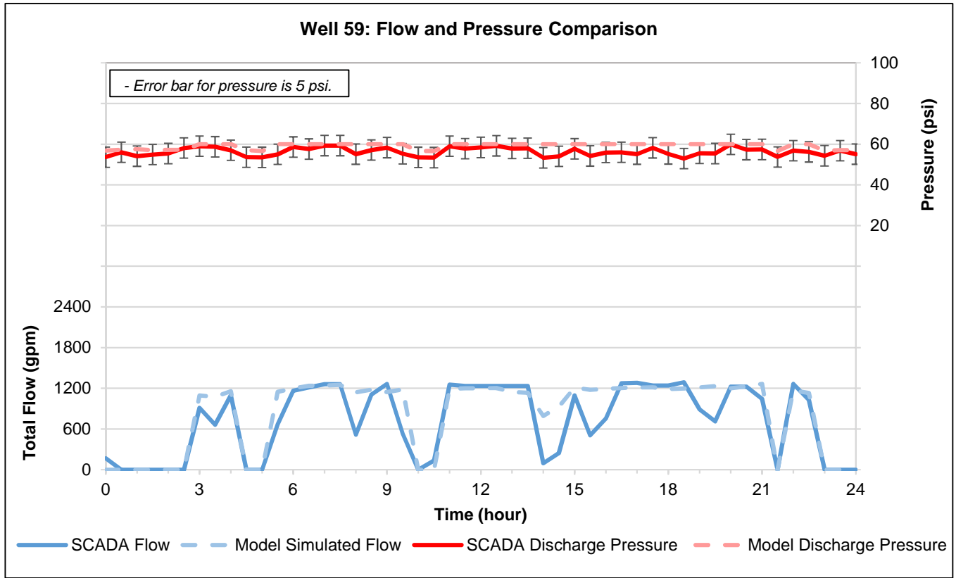
Figure 18. Well 59 and 62 December 15, 2015
